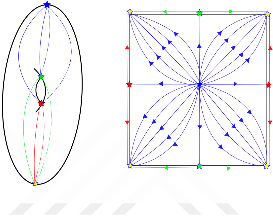
Figure 2.7: Compactification of the moduli space of S^1 \times S^1 .
