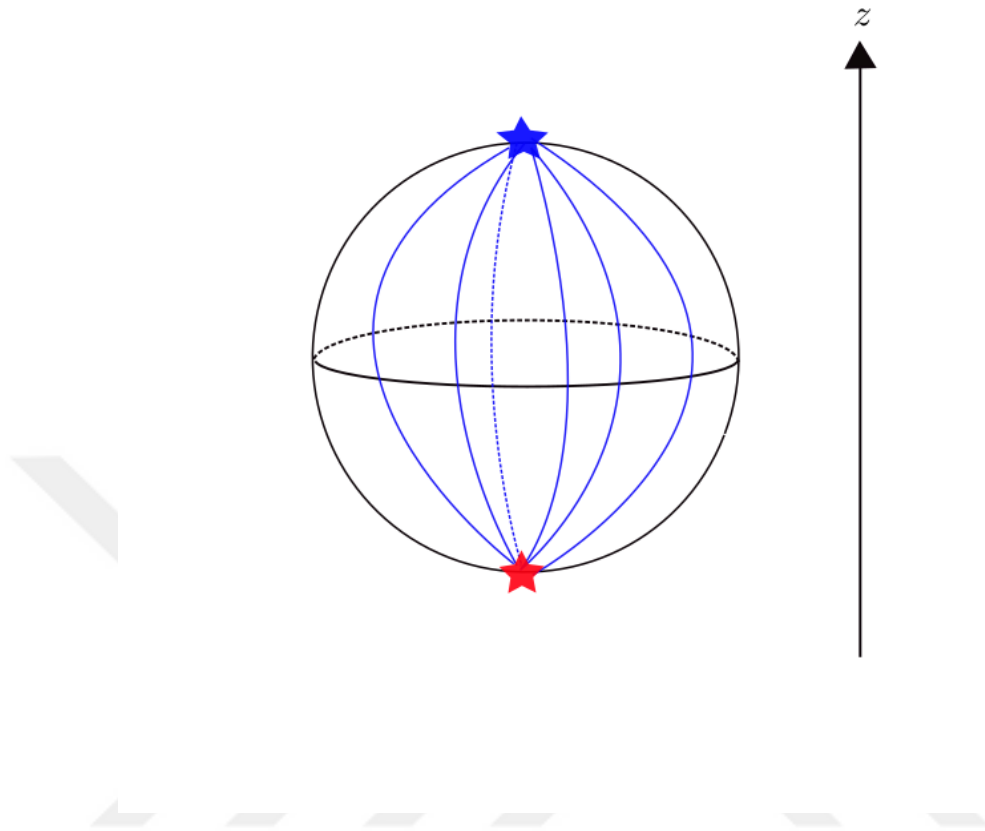
Figure 2.5: Flow lines in S^2 .
