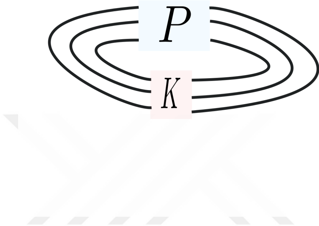
Figure 12.3: After the cancellation trick.
