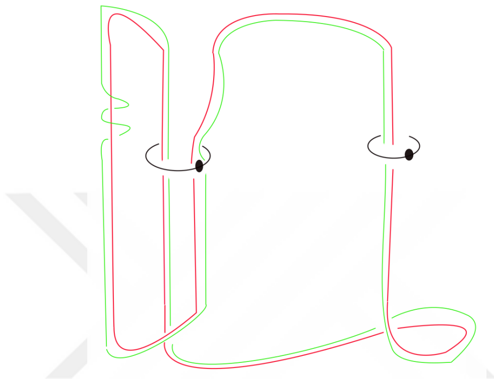
Figure 7.6: A longitude (framing) of a knot.
