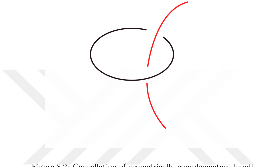
Figure 8.2: Cancellation of geometrically complementary handles.
